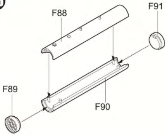
M260 Hydra Rocket Pods 7round
