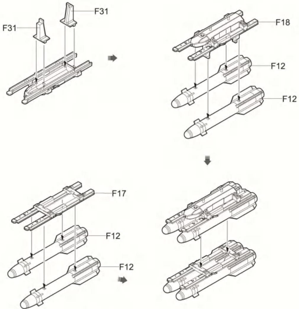
AGM-114A "Hellfire"
